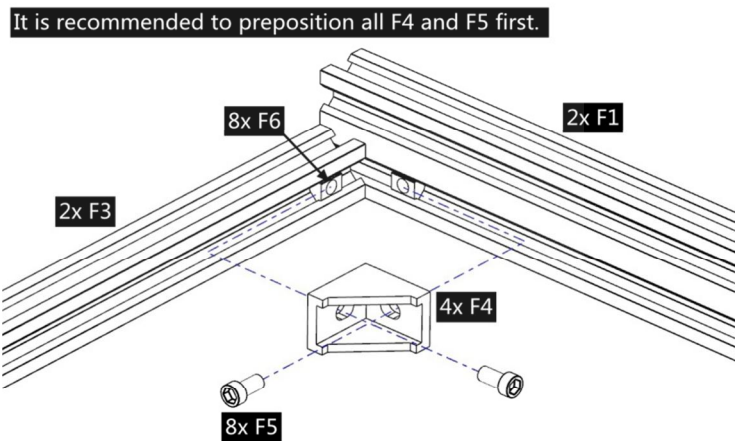
12. Connect F1 and F3 with F4 and F5. Please notice the flatness of the whole framework. It is recommended to preposition all F4 and F5 first. Lay the frame flat on a flat
