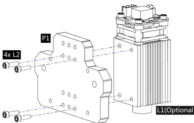
1. Assemble Laser L1 (Optional) and P1.
