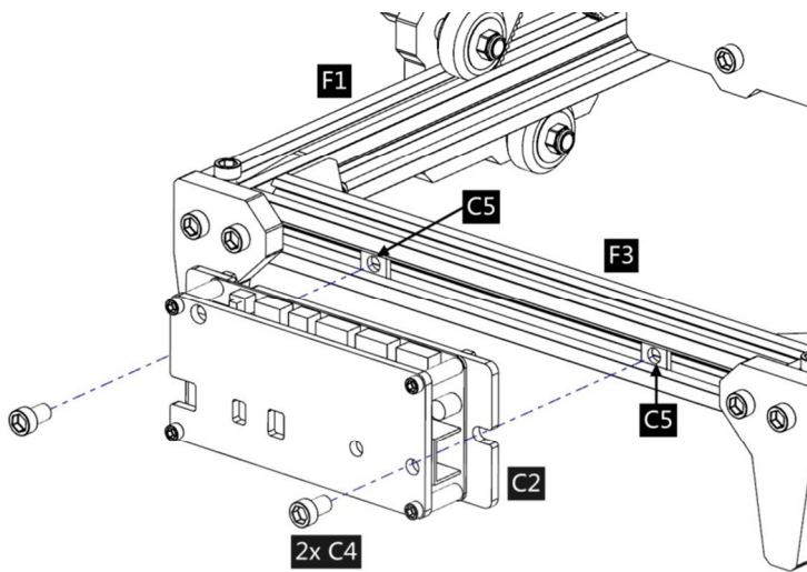
19. Assemble the Control-Part to the rear profiles F3.
