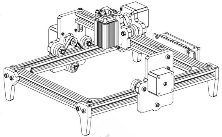
20. Final assembly completed.
