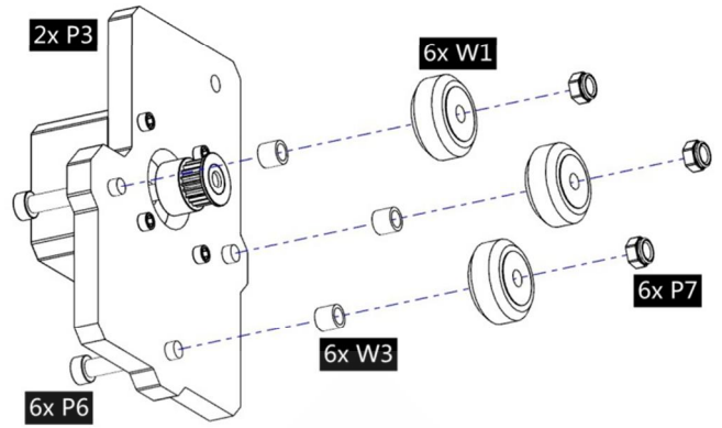
8. Assemble W1 and W3 to P3. Assemble 2 sets symmetrically.
