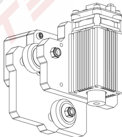
4. Assembly completed. This part is named X-Part.
