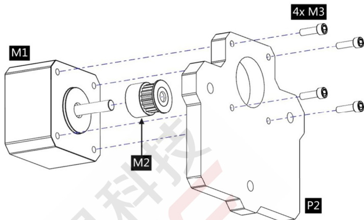
2. Assemble M1, M2 and P2.
