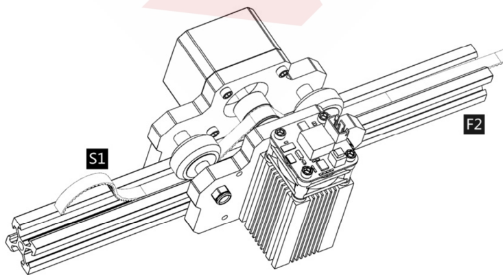
5. Slide F2 into X-Part. And pass S1 through the synchronous pulley and the Flat pulley as shown in the figure.
