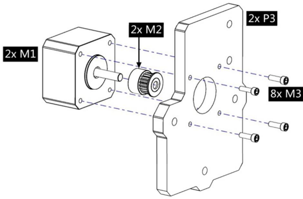
7. Assemble M1, M2 and P3. Assemble 2 sets symmetrically.
