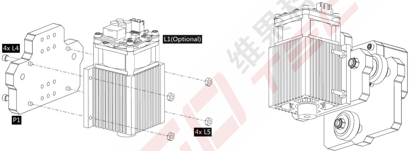
1. Assemble Laser L1 (Optional, include L4 and L5) and P1.
